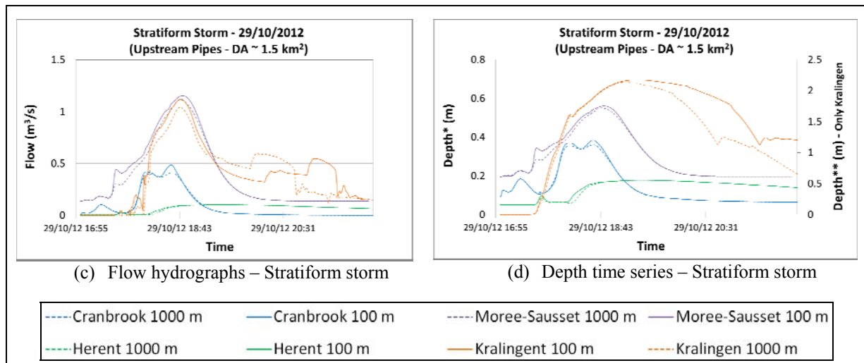
Figure 2: Response hydrographs and water depths at the downstream end of the upstream pipes selected for analysis at each pilot location (with drainage area (DA) \sim 1.5 \text{ km}^2 ). The solid lines correspond to the 100 m resolution outputs and the dashed lines to the 1000 m ones. * Water depth scale used for depths observed in Cranbrook (UK), Morée-Sausset (FR) and Herent (BE) pilot locations; **Water depth scale used for Kralingen (NL) pilot location.
