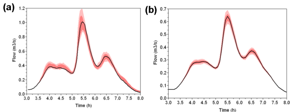
Figure 3. Simulated flow with raw radar data (black), Q_{0.25} and Q_{0.75} (dark colour), Q_{0.1} and Q_{0.9} (light colour) for the outlet of the Kodak catchment. (a) Multi-Hydro 10 m; (b) 1D model (adapted from Gires et al., 2013)
