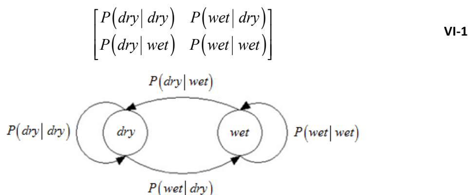
Figure 20: Schematization of a first order two state Markov chain (adapted from Hocaoglu, 2011)
