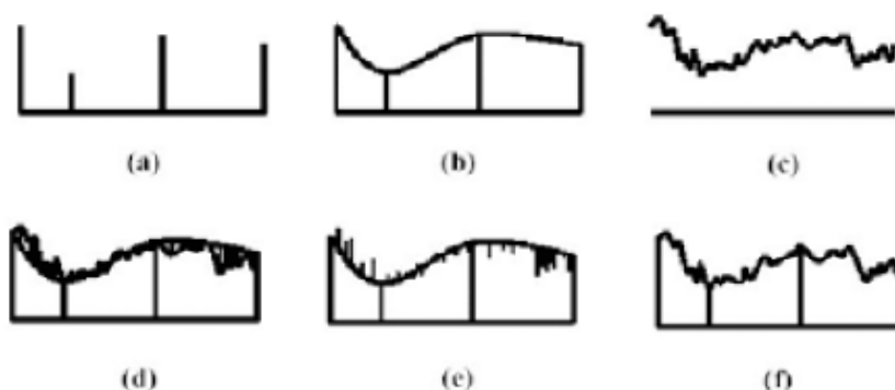
Figure 11: Conditional merging scheme: the TBR rainfall information (a) is spatially interpolated by the kriging method (b), the radar based rainfall information is shown in (c). The two are compared in (d) and the differences of the radar estimates with the kriging results are shown in (e). These differences are applied to the kriging results to incorporate the spatial rainfall variability as observed by the radar (adapted from Pegram and Sinclair, 2004)
