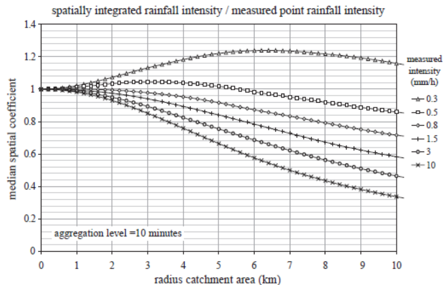
Figure 23: Median values for the areal correction coefficients (type I) for an aggregation level of 10min as a function of the measured rainfall intensity at the central point location (after Vaes et al., 2005)
