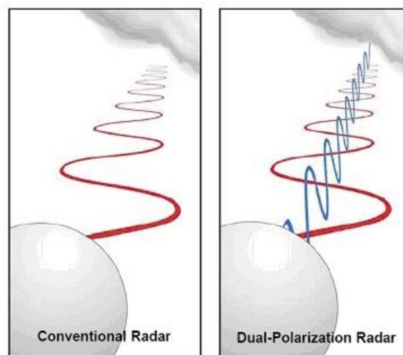
Figure 2: Working principle of a conventional (single, horizontal polarization) radar versus a dual polarization (horizontal and vertical) radar (Source: NOAA)
