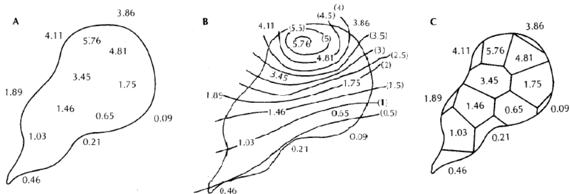
Figure 25: Rainfall interpolation methods based on gauges: A: a drainage basin with rain gauges (their position is marked by their respective measurement values), B: the spatial rainfall distribution based on the isohyetal method and C: the spatial rainfall distribution based on the Thiessen method (adapted from Fetter, 1994)
