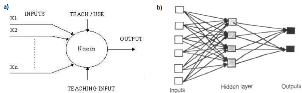
Figure 19: Artificial neural network schematization: a) representation of one single neuron and b) representation of a simple feed-forward neural network architecture (adapted from Stergiou and Siganos, 1997)
