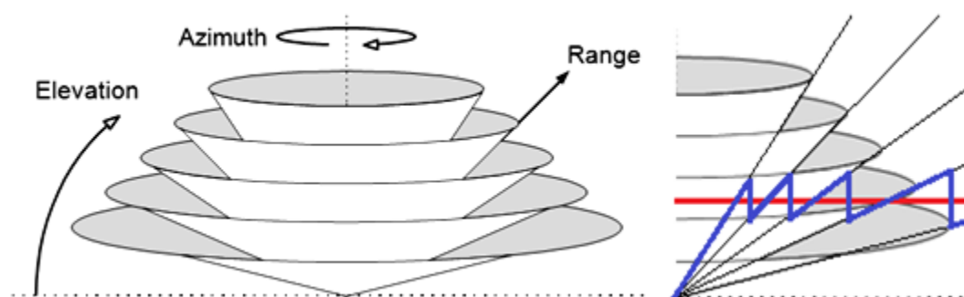
Figure 9: a) Radar scanning strategy: example of scans at different elevation levels (adapted from EG-CLIMET MediaWiki) b) Composing a CAPPI from the scans at different elevation levels, the Pseudo-CAPPI is marked in blue and uses the closest scan available for a given height (marked with the red line)
