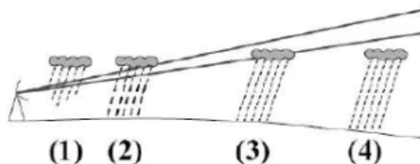
Figure 4: Several problems caused by the measuring height and volume of the radar, such as evaporation (1), condensation or coalescence (2), partial beam filling (3) or even overshooting of the rain (4) (after Delobbe, 2006).
