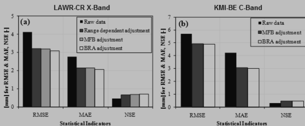
Figure 27: Comparison of the performance of the radar adjustment procedures: a) LAWR-CR X-band and b) RMI C-band, comparison of the statistical indicators for summer (adapted from Shrestha et al., 2012)
