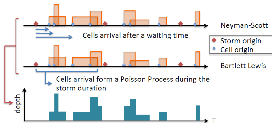
Figure 12: Schematisation of the Neyman-Scott and Bartlett-Lewis model (adapted from Paschalis, 2012)
