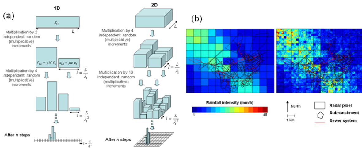
Figure 14: Rainfall downscaling a) Illustration of a cascade process in 1D and 2D (adapted from Gires, 2012), b) an example of the spatial downscaling based on real data (adapted from Gires et al., 2012b)
