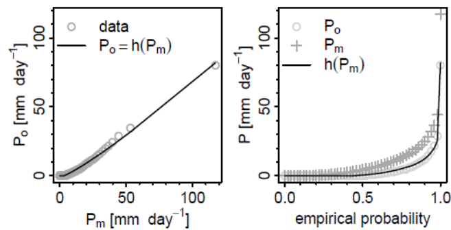
Figure 18: Example of the Quantile mapping method: left: a quantile quantile (QQ-) plot of observed ( P_o ) and modeled ( P_m ) precipitation and a transformation function ( h ) to map the quantiles together, right: the empirical cumulative distribution function (CDF) of the observed modeled and transformed ( h[P_m] ) precipitation (after Gudmundsson et al., 2012).
