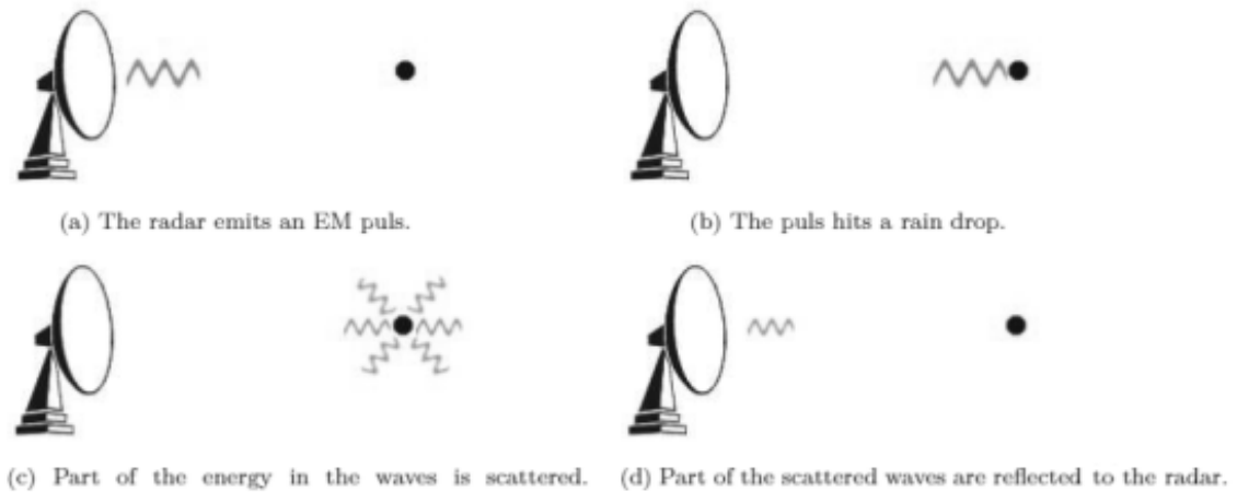
Figure 1: Working principle of a weather radar (after Cain, 2002)
