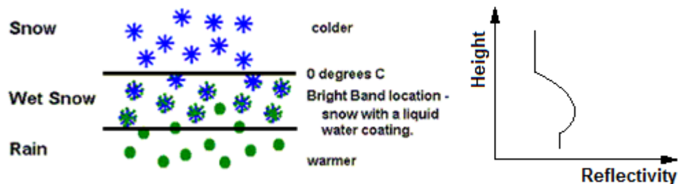
Figure 5: Principle of bright band formation below the 0°C line: left) microphysical formation of the bright band, right) consequences on the radar VPR, idealized reflectivity vs. height diagram (adapted from the North Carolina State University website)
