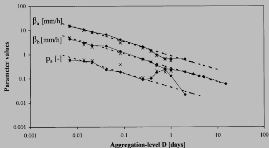
Figure 22: Scaling properties of the parameters of the two-component exponential distribution (after Willems, 2000)
