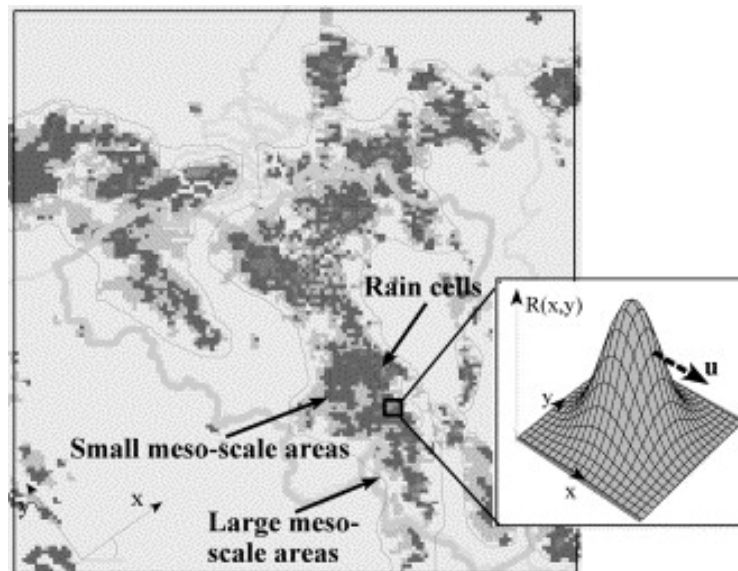
Figure 13: Rainfall distributed over Belgium and the Gaussian-shaped rainfall cells (after Willems, 2001b).
