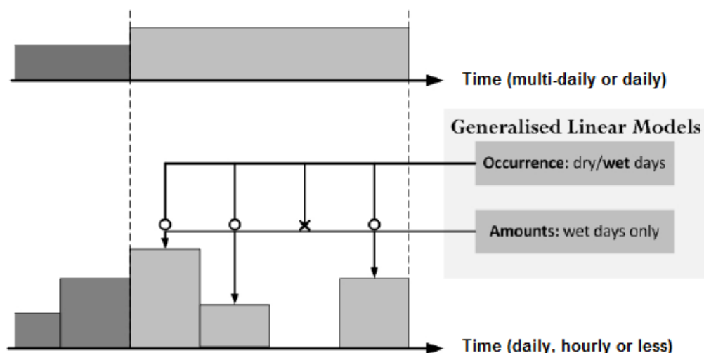
Figure 17: Schematization of the GLM downscaling method with the two phase approach, consisting of the occurrence and the amounts models (adapted from Wang, 2012)
