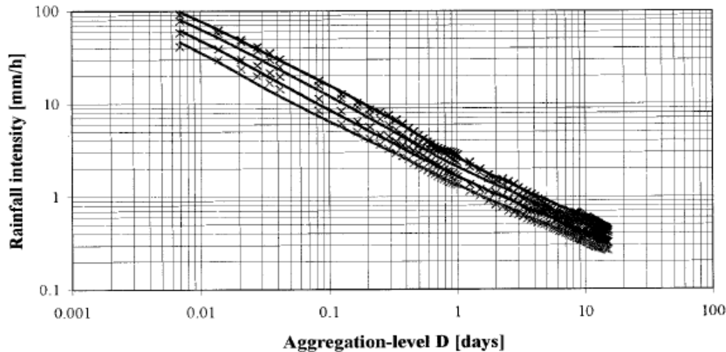
Figure 21: IDF-relationships for return periods of 27, 9, 2.7 and 1 years; comparison of calibrated IDF-relationships (full lines) with observations (source: Willems, 2000)
