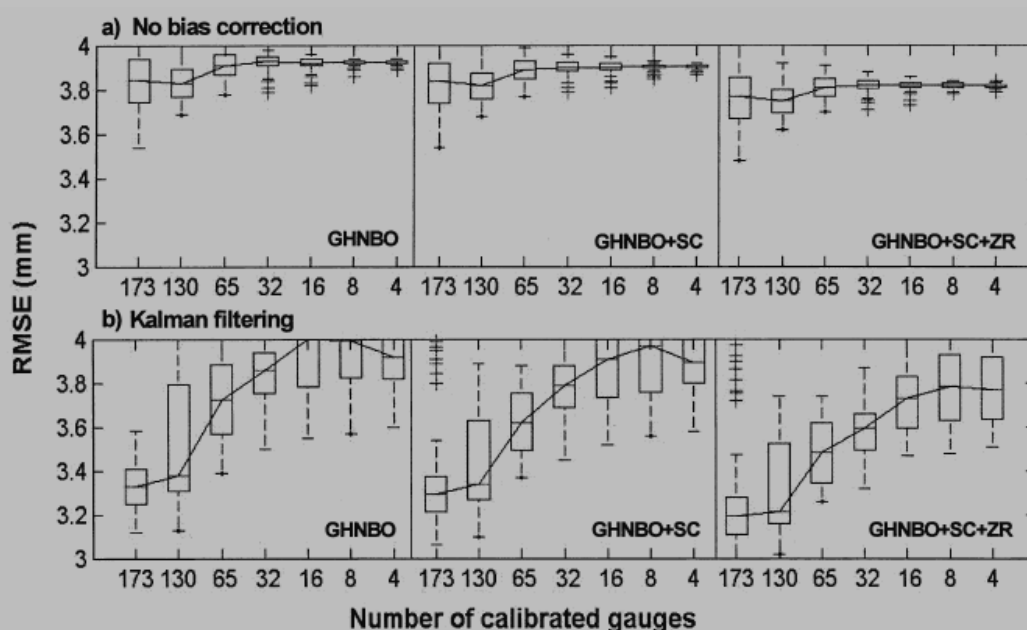
Figure 26: Validation of the RMSE for radar based rainfall QPEs for a different number of calibrated gauges and different error correction strategies with a) no bias adjustment and b) Kalman filtering. Note: "GHNBO" denotes correction of ground clutter, hail, and noise and range-dependent bias resulting from bright band and different observation altitude, "SC" denotes correction of range-dependent bias resulting from increases in observation volume (scaling correction) and "ZR" denotes correcting for variation of Z-R relationship for convective and stratiform rainfall (storm classification) (Adapted from Chumchuan et al., 2006).
