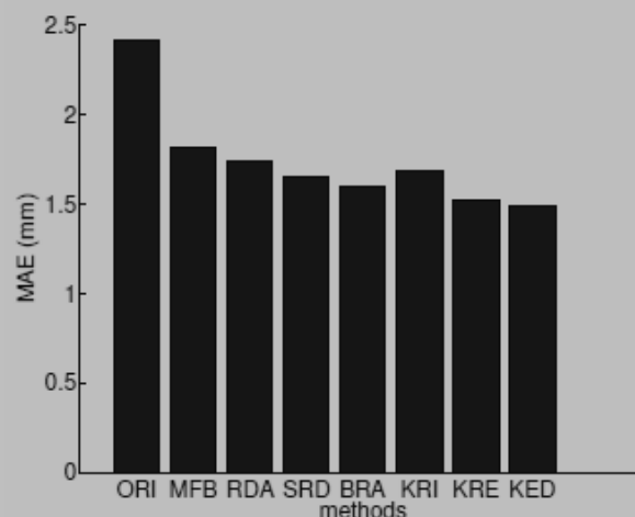
Figure 28: Comparison of the performance of the radar adjustment procedures (after Goudenhoofdt and Delobbe, 2009)
