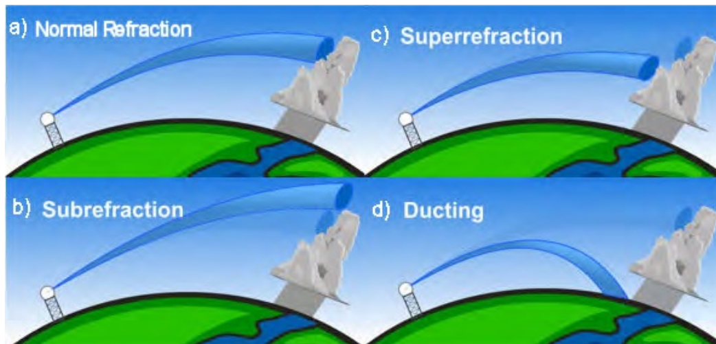
Figure 7: Radar beam propagation pattern under different atmospheric conditions: a) normal refraction, b) sub-refraction, c) super-refraction and d) trapping or ducting (after Bech et al., 2012)
