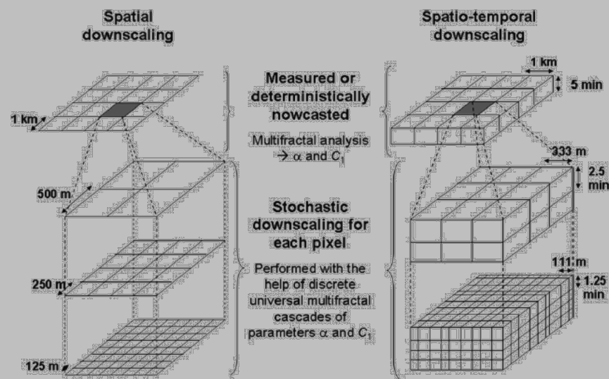
Figure 15: Illustration of the spatial (left) and spatio-temporal (right) downscaling techniques
