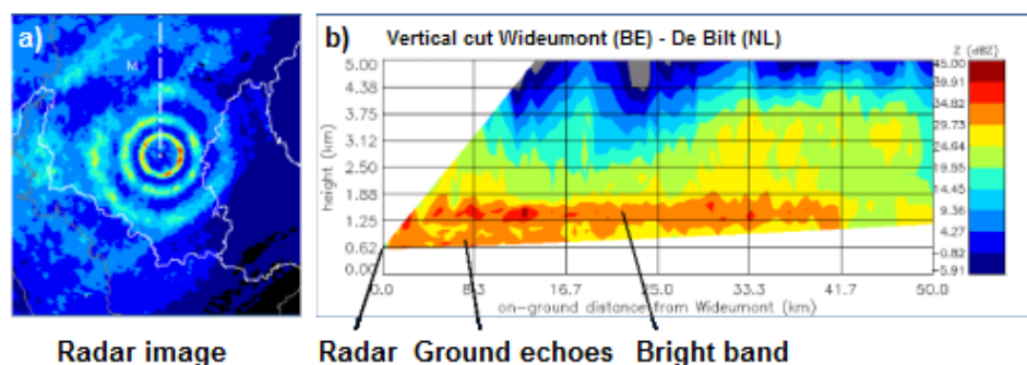
Figure 6: Bright band phenomenon in radar images: a) Radar image from Wideumont (Belgium) affected by Bright band, b) vertical cut from the same radar image from the radar to the north (towards De Bilt, the Netherlands) (source: RMI)
