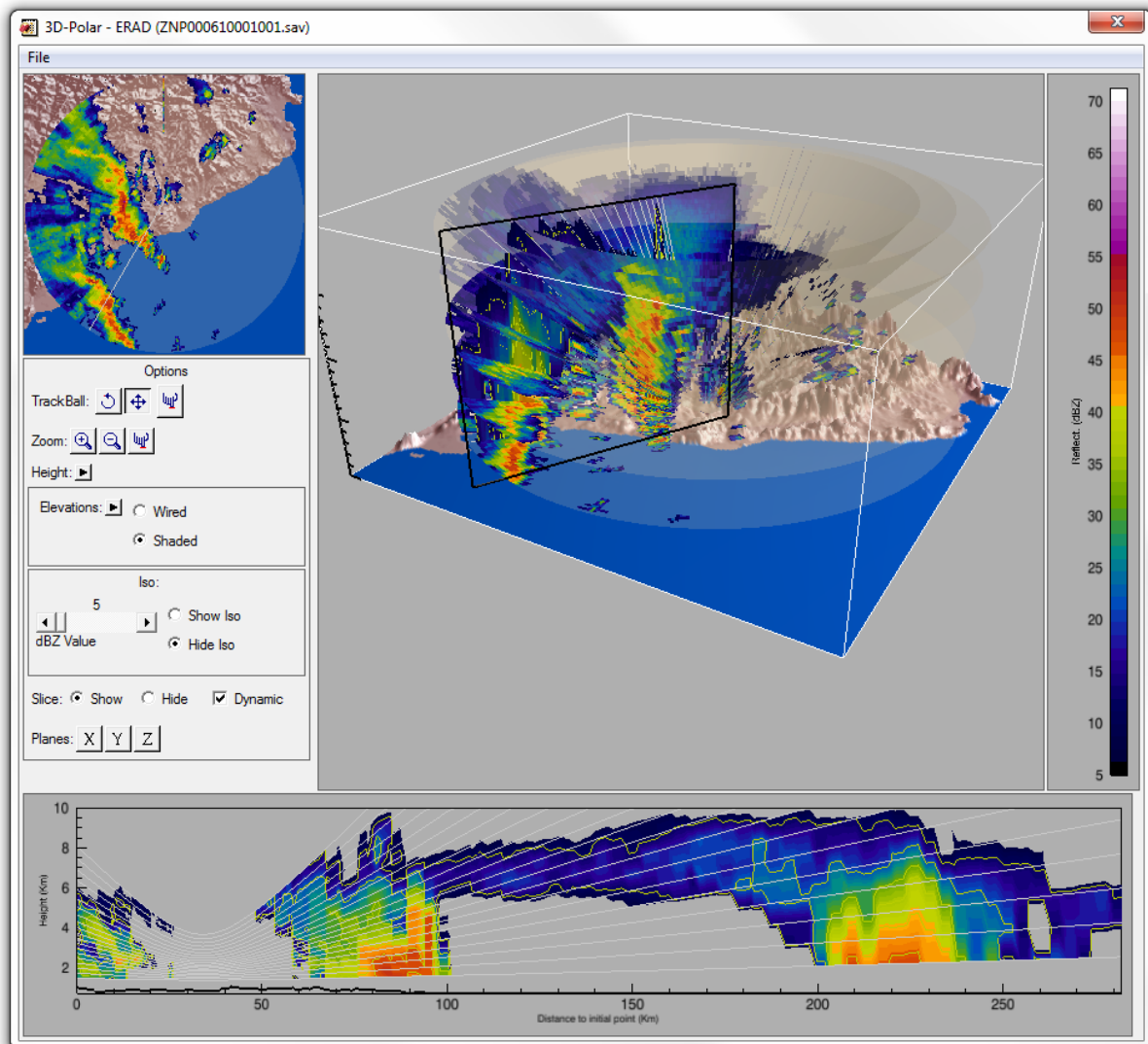
Figure 10: A figure illustrating the scanning strategy: (top right corner) the different elevation scans - PPI's, (top left corner) the pseudo-CAPPI and (bottom) a cross section through 2 convective lines (the cross section is marked by the white line in the pseudo-CAPPI and the black window in the PPIs). (Visualized with software provided by CRAHI - Center of Applied Research on Hydrometeorology - Polytechnical University of Catalunya)
